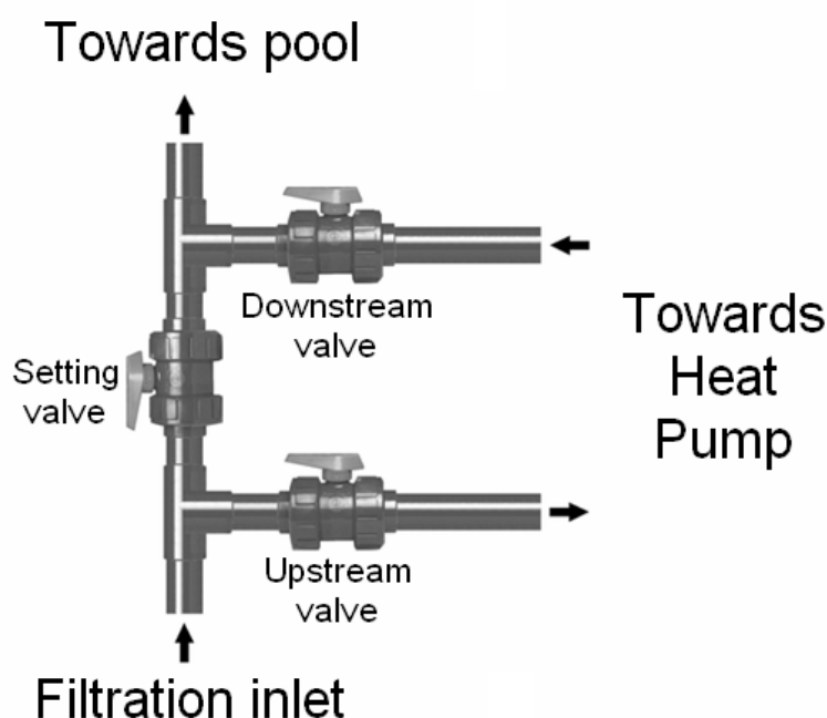
By-pass diagram
